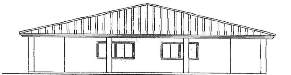
FACHADA PRINCIPAL
